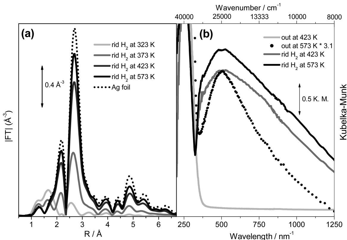
Figure 7. Effect of H 2 reduction at increasing temperatures on the k^2 -weighted, phase-uncorrected FT of the EXAFS spectra and on the UV-vis spectra, parts a and b respectively. For sake of comparison, the spectrum of Ag foil reference compound is included in part a, while (from Figure 5) those of the Ag-ETS-10 samples activated at 423 and 573 K (the latter multiplied by a factor 3.1 to match the intensity of the plasmon peak of the sample reduced in H 2 at 423 K) are added in part b.
