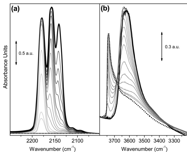
Figure 3. Evolution of IR spectra of CO adsorbed, at 100 K, on Ag-ETS-10 outgassed in a vacuum at 423 K down to 10^{-4} Torr (dotted black spectrum) upon increasing equilibrium pressure (up to P_{CO} = 50 Torr, black bold spectrum). The light gray spectra (not reported in part b) refer to the lowest P_{CO} (where only Ag + sites are engaged), and dark gray spectra refer to intermediate P_{CO} (where also O–H groups are engaged), while black curves refer to the highest P_{CO} values (where liquidlike CO is formed in the zeolitic cages). Part a reports background subtracted spectra and refers to the \nu(\text{CO}) stretching region. Part b refers to the \nu(\text{OH}) stretching region.
