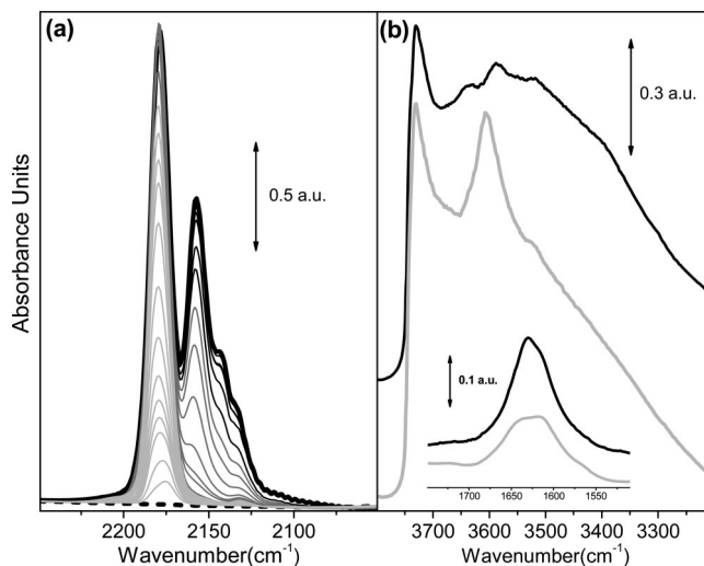
Figure 8. (a) Evolution of IR spectra in the C-O stretching region, of CO adsorbed, at 100 K and increasing P_{CO} (up to P_{CO} = 50 Torr, black bold spectrum) on Ag-ETS-10 reduced in H 2 at 423 K and successively oxidized in O 2 at the same temperature (dotted black spectrum). Gray thin spectra refer to intermediate P_{CO} values. The same color code is used as in Figure 2. (b) IR spectra in the \nu(OH) region of Ag-ETS-10 reduced in H 2 at 423 K (gray curve, vertically shifted for clarity) and of the same sample subjected to a successive oxidation treatment in O 2 at 423 K (black curve). The inset reports the same spectra in the \delta(OH) region.
